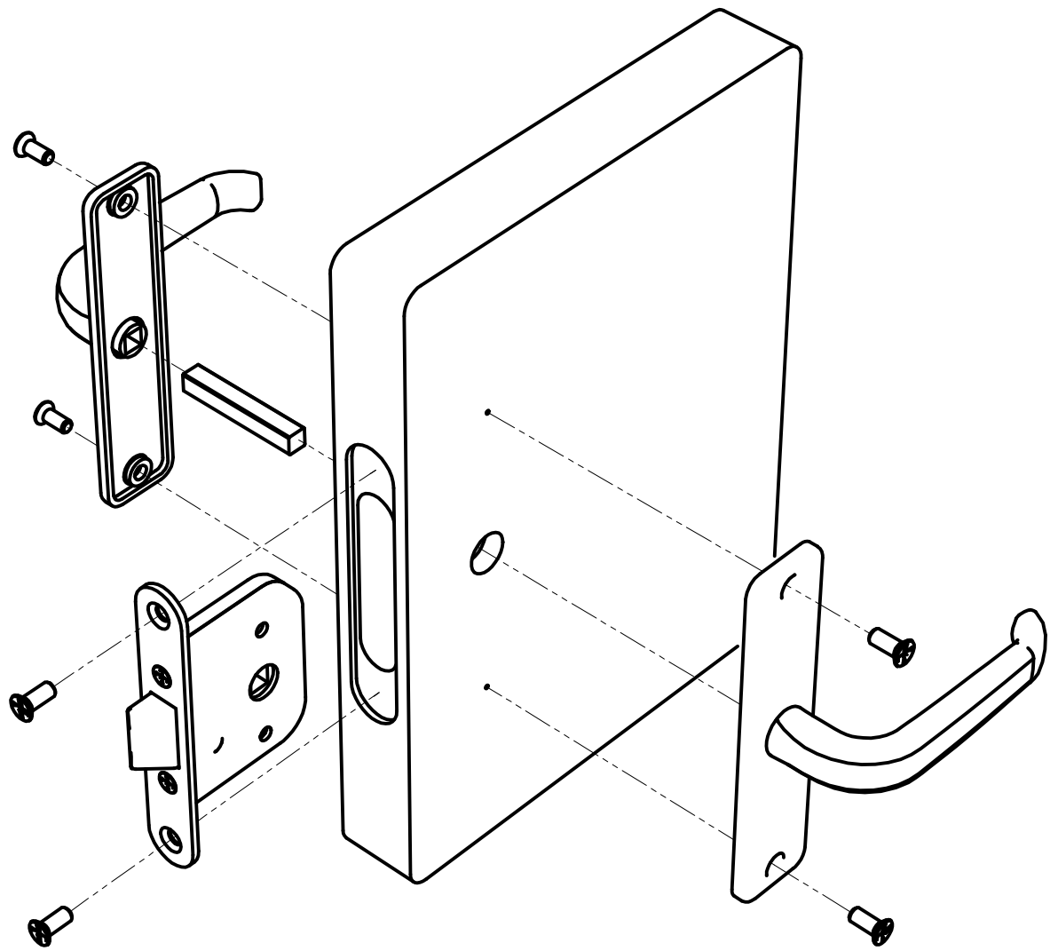
SMALL - Swing Door Lock Installation
